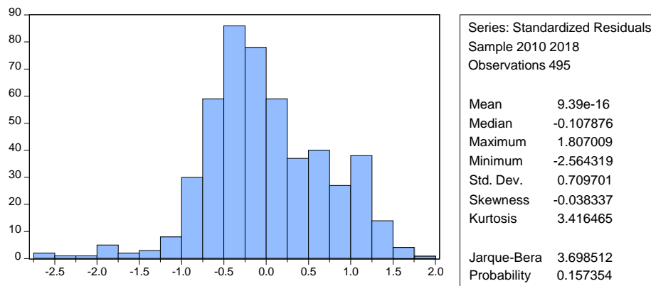
Figure 1 Normality Test (DV: Firm Value)
