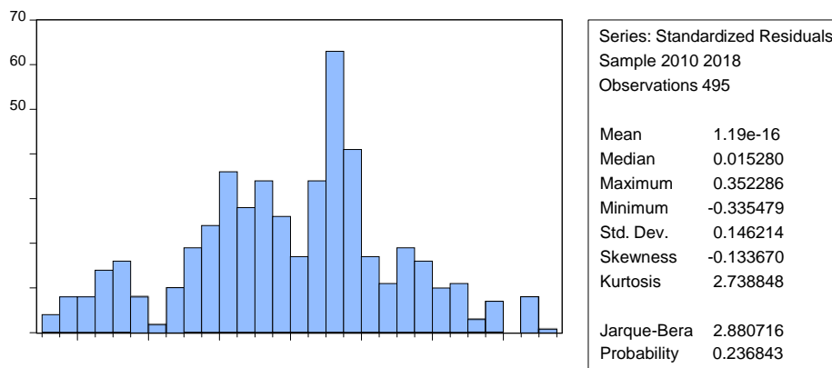
Figure 2 Normality Test (DV: CSR)
